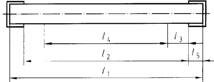
Figure 4: Specimens for hydrostatic pressure resistance test
